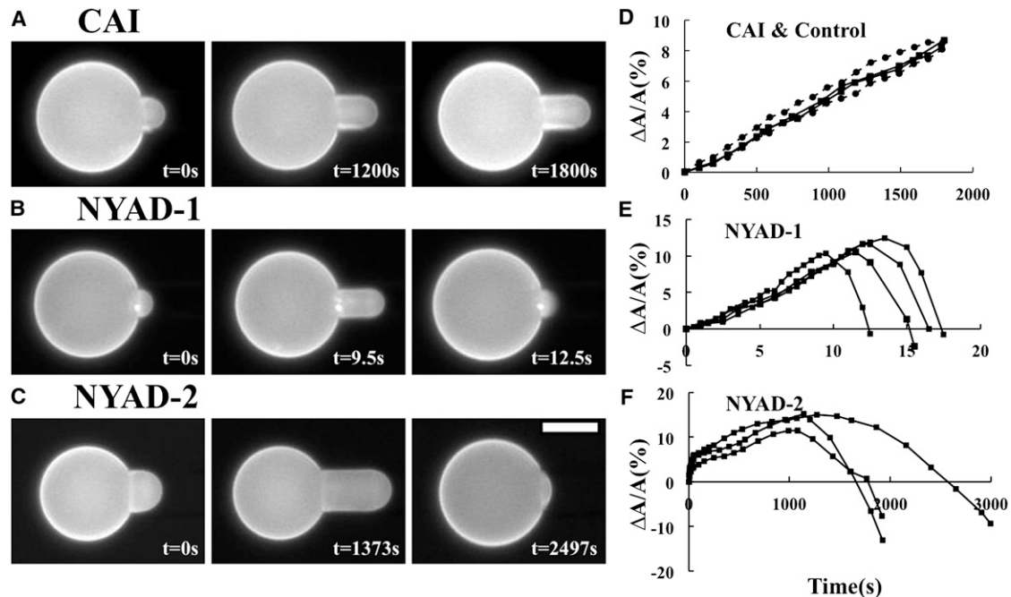
FIGURE 2 An aspirated GUV of DOPC (and 0.5% molar ratio of Rh-DOPE) was introduced into a solution containing 8 \mu\text{M} CAI (A), 8 \mu\text{M} NYAD-1 (B), or 8 \mu\text{M} NYAD-2 (C) at pH 7. The length of the GUV protrusion into the micropipette, L_p , was measured at regular time intervals. For the purpose of comparison, \Delta L_p was converted to the fractional area change \Delta A/A by the relation \Delta A = 2\pi R_p(1 - R_p/R_v)\Delta L_p . (A) With CAI, the protrusion length increase is similar to the control runs without peptides, as shown in (D). (B and C) With NYAD-1/NYAD-2, the protrusion length increased initially. After the protrusion length reached a maximum, it steadily decreased; this indicates pore formation. Scale bar = 25 \mu\text{m} . Experiments A, B, and C were repeated several times with similar results. (D) The protrusion length change was converted to \Delta A/A for CAI (square dots, solid lines) compared with controls (round dots and dashed lines)—2 runs are shown for each. The osmolalities of the internal and external solutions of GUVs were initially balanced. The protrusion length increase in a control was due to water evaporation from the external solution. (E) \Delta A/A vs. time for 4 runs of the NYAD-1 experiment. (F) \Delta A/A vs. time for 3 runs of the NYAD-2 experiment. In (E and F), a decreasing \Delta A/A is used to indicate pore formation, not a decrease in membrane area.
