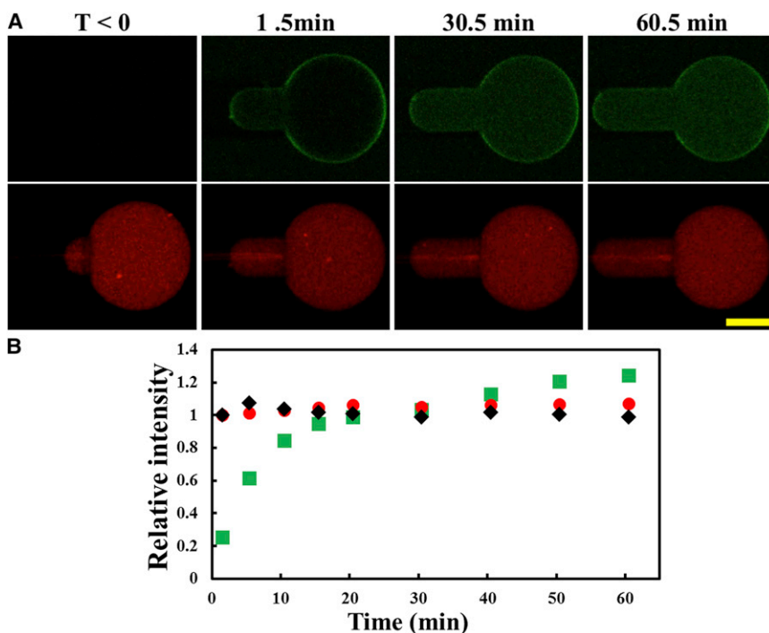
FIGURE 4 (A) Confocal images of an aspirated GUV (DOPC) containing a pH 9 solution and 10 \mu\text{M} TRSc (red) in the lumen, first in the control chamber ( t < 0 ) and then transferred to the observation chamber (time 0) containing a solution of 2 \mu\text{M} NYAD-2 (green) at pH 7. The binding of NYAD-2 (the green intensity on the GUV boundary increased with time) caused the membrane expansion (protrusion length increase) with no molecular leakage. (The bright, thin, horizontal red bar on the micropipette was an optical artifact.) Scale bar = 20 \mu\text{m} . (B) Relative intensities of fluorescence: Red for TRSc inside the GUV (normalized to one at t = 0 ); Black for the corrected solution intensity of NYAD-2 outside the GUV, I_O^c (also normalized to one at time = 0); Green for the corrected intensity of NYAD-2 inside the GUV divided by the corrected intensity outside averaged over time, I_i^c (and divided by 1.78 due to the pH 9 effect): I_i^c / (I_O^c * 1.78) . Note that the corrected intensity inside the GUV exceeded the corrected outside intensity after \sim 30 min.
